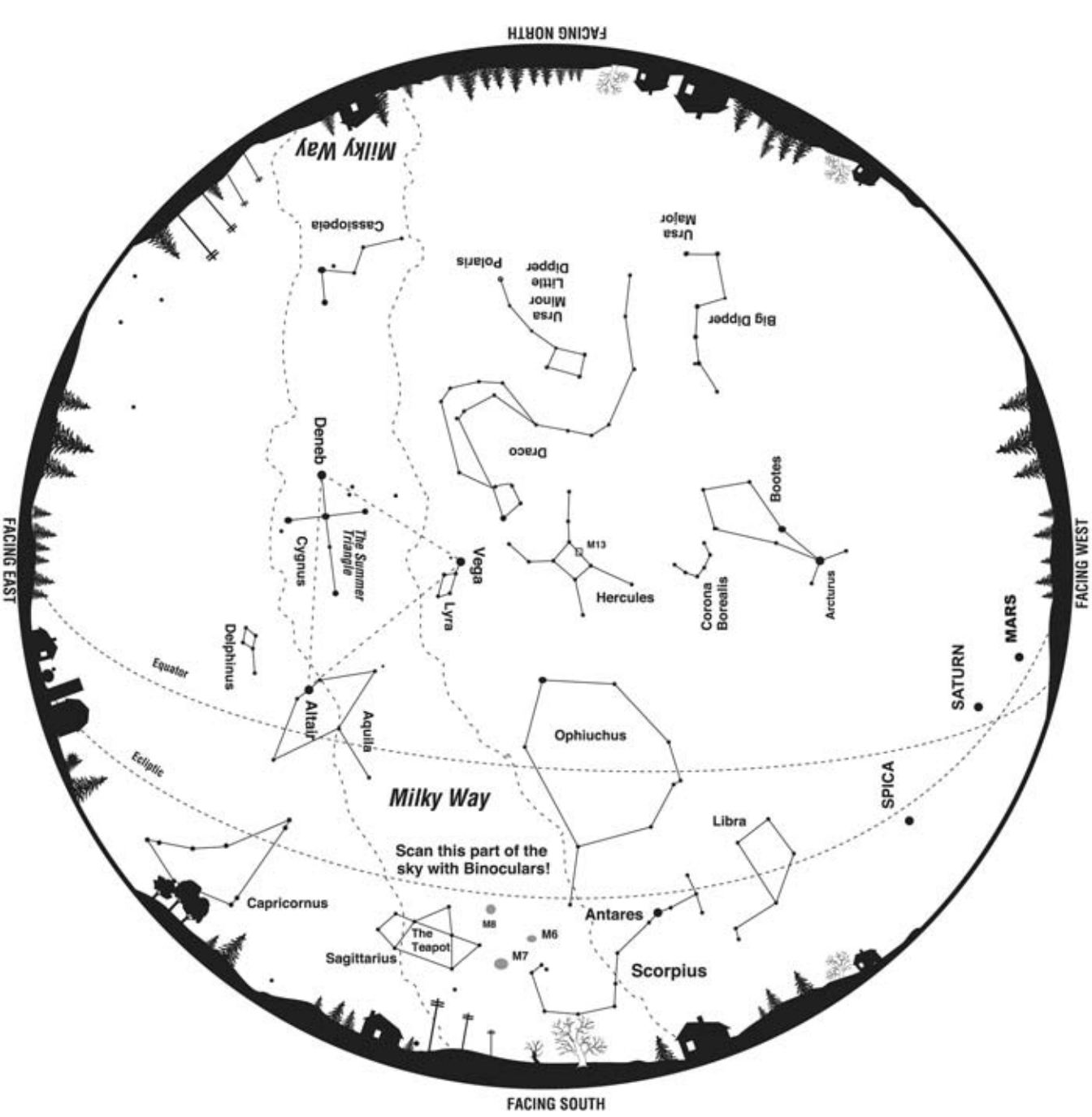
JULY ALL-SKY CHART EARLY JULY-11PM LATE JULY-9PM
