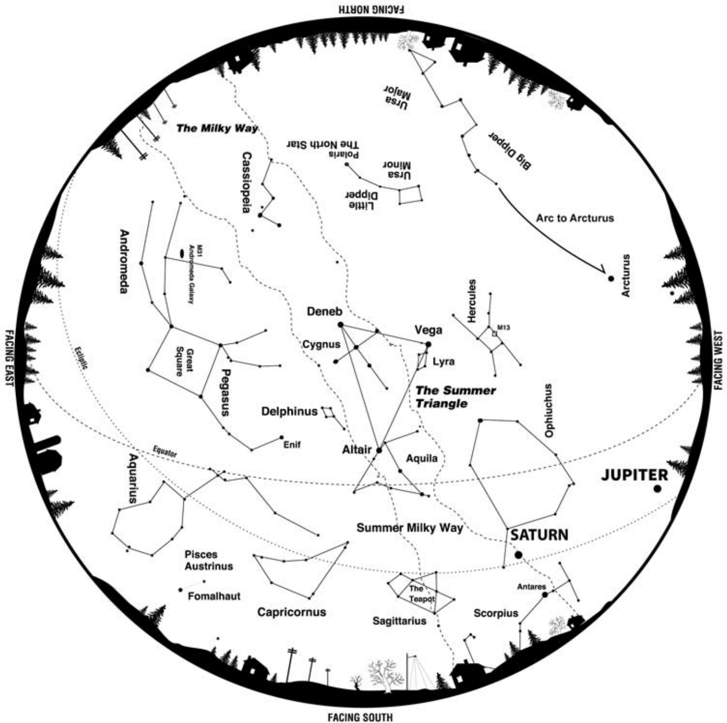
SEPTEMBER ALL-SKY CHART EARLY SEPTEMBER – 9:30PM LATE SEPTEMBER – 8PM
